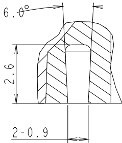
"B" Detail
