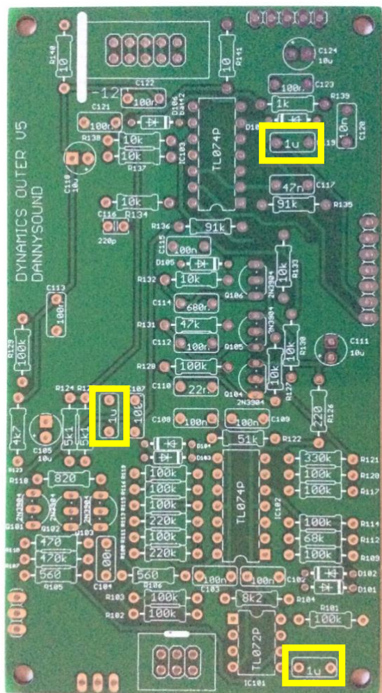
28) – 3 x 1u film (C101, C106, C119)
