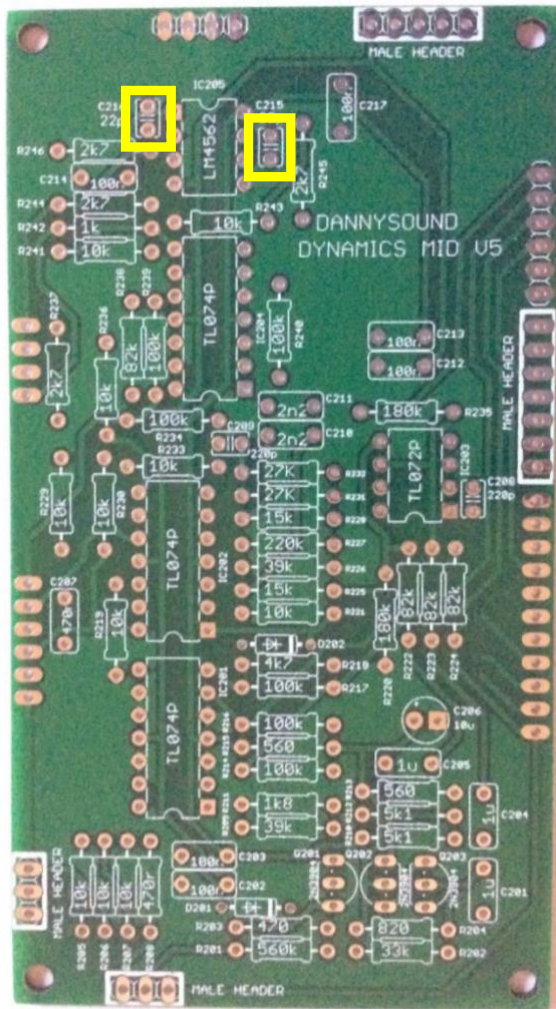
60) – 2 x 22p ceramic (C215, C216)
