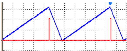
Figure 10b: EOR Trigger output Width of trigger is 4ms
