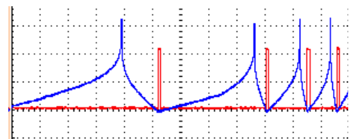
Figure 11b: EOF Trigger output Width of trigger is 4ms
