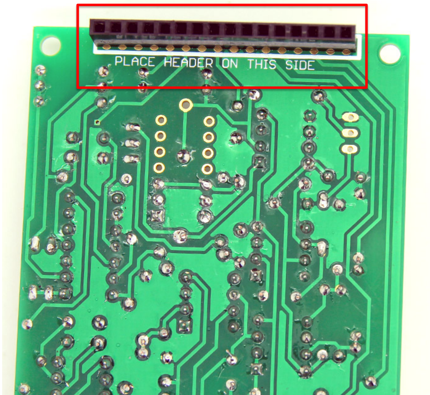
30 – Female connector
