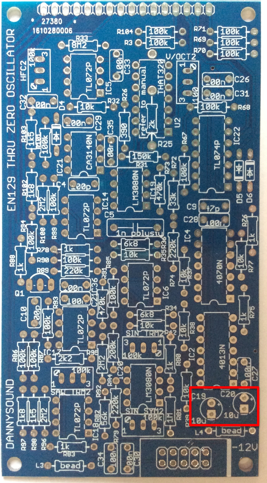
29 – 2 x 10uF capacitor - orientation is vital, the longer lead on the component should go to the circular pad marked with a plus '+' on the PCB. Note the component has a grey stripe on the cylindrical body on the minus side.
