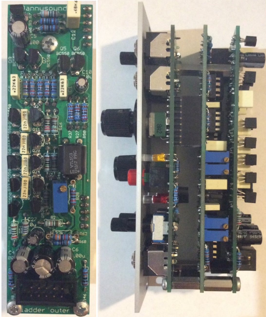
85) – Attach the outer board and screws
