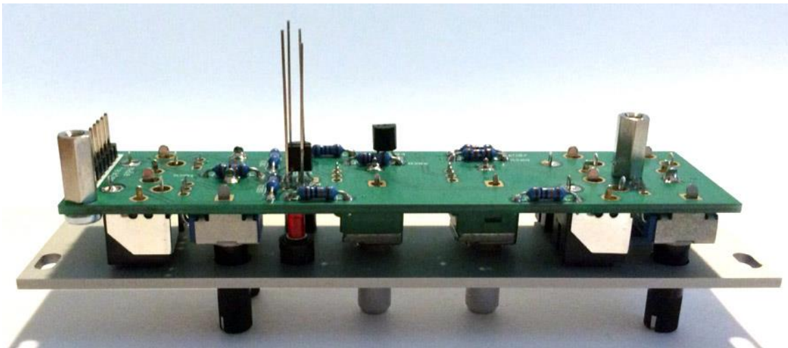
73 - Solder one leg of each of the LEDs, you can then reflow the solder to that pin while holding the LED legs to position it nicely against the light pipes.
