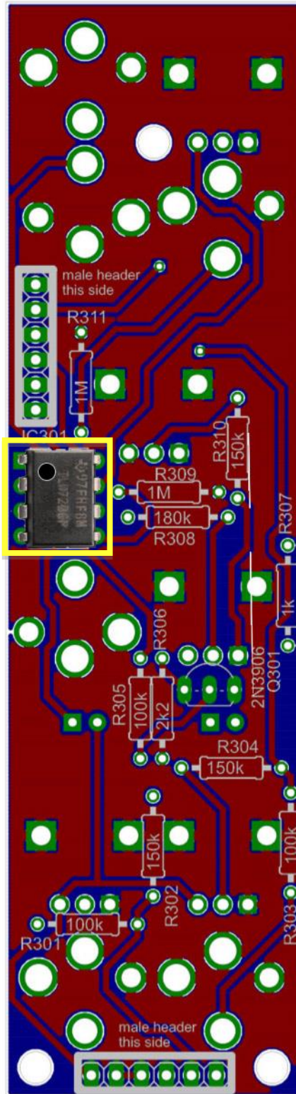
63 - 1 x TL072 opamp - orientation is vital, for this opamp match the dot with the notch on the PCB silkscreen and IC Socket
