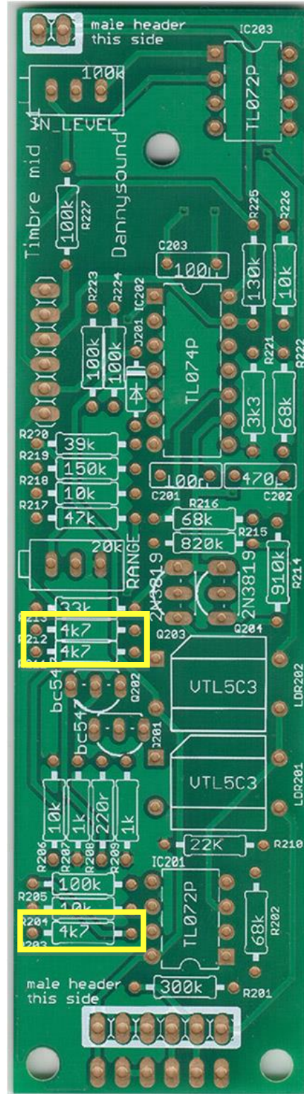
28 - 3 x 4k7 (R203, R211, R212)
