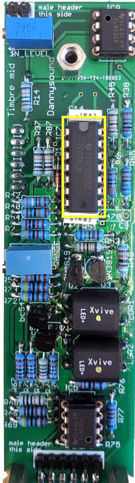
54 - 1 x TL074 opamp - orientation is vital, for this opamp match the notch on the chip with the notch on the PCB silkscreen and IC socket
