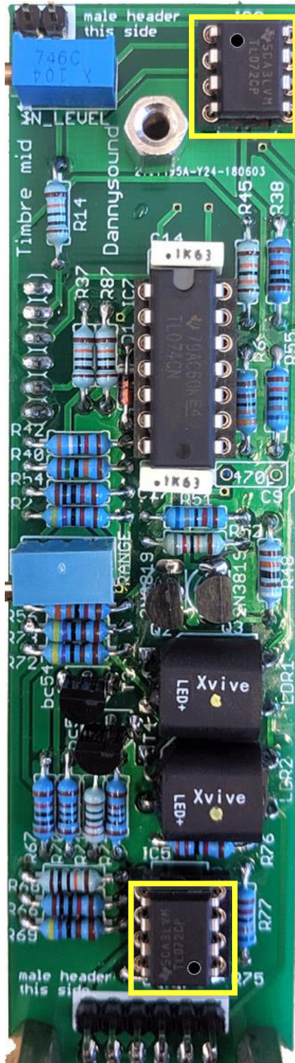
53 - 2 x TL072 opamps - orientation is vital, for these opamps match the dot with the notch on the PCB silkscreen and IC socket
