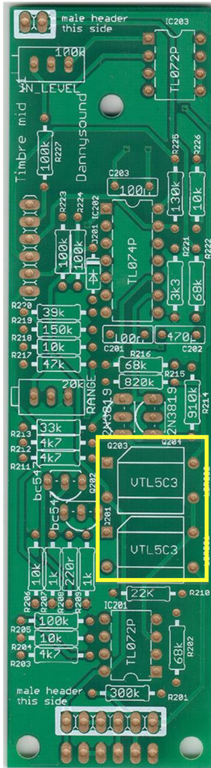
50 - 2 x VTL5C3 Vactrols - Note: orientation matters -the sloped edge of each Vactrol must line up with the sloped edge on the PCB silkscreen.
