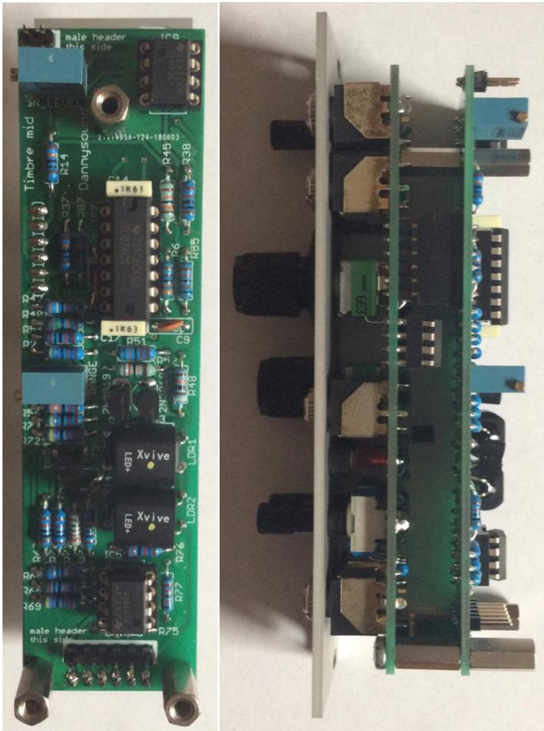
76 - Attach the mid board to the pot board using the 3 x Male to Female 12mm standoffs.
