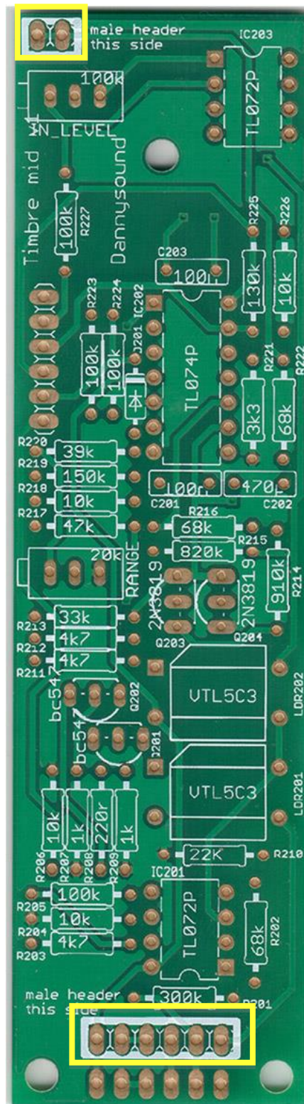
51 - 1x6 pin and 1x2 pin male header - these headers are placed on the same side as the rest of the components on this PCB
