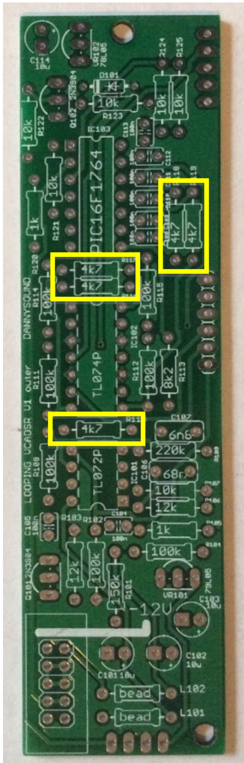
9) - 5 x 4k7 (R110, R116, R117, R118, R119)
